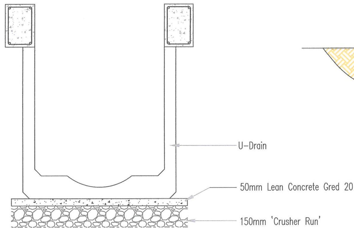
U-Drain
