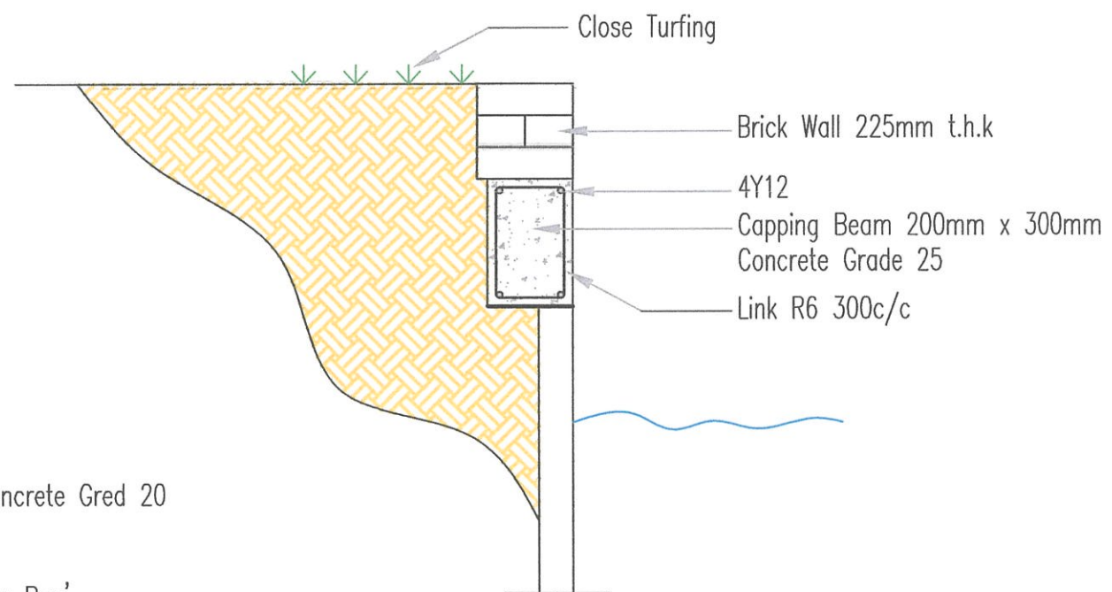
Details Capping Beam
